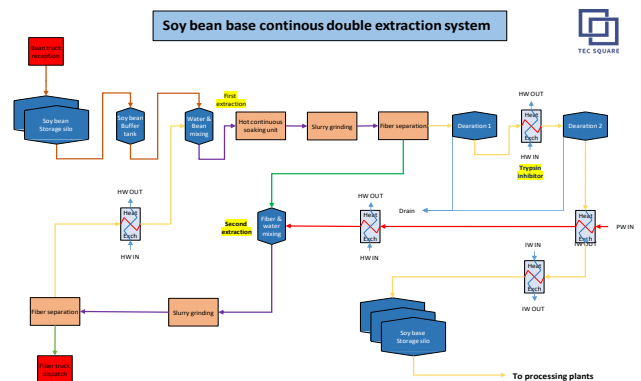
Schematic for a typical Soy Milk Extraction Plant
